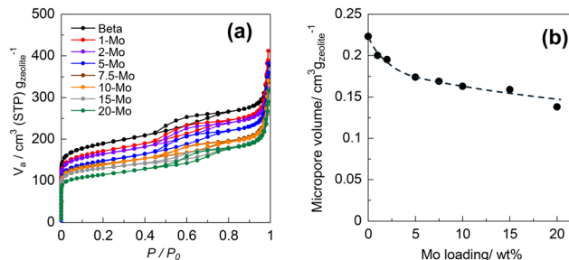
Fig. 3 (a) \text{N}_2 adsorption-desorption isotherms of Mo-loaded beta zeolite catalysts and (b) influence of Mo loading on microporous volume.
