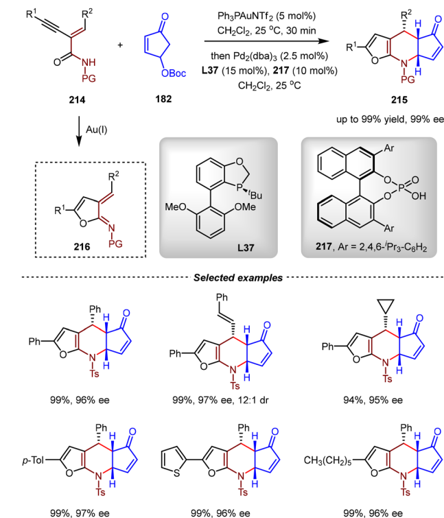
Scheme 45 Asymmetric synthesis of furo[2,3- b ]pyridines by sequential Au(I) and Pd(0)/chiral phosphoric acid catalysis.
