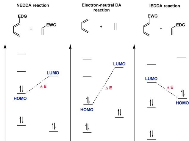
Scheme 1 Classification of Diels–Alder reactions. NEDDA reactions, normal-electron-demand Diels–Alder reactions; IEDEDA reactions, inverse-electron-demand Diels–Alder reactions; HOMO, highest occupied molecular orbital; LUMO, lowest unoccupied molecular orbital; EDG, electron-donating group; and EWG, electron-withdrawing group.
