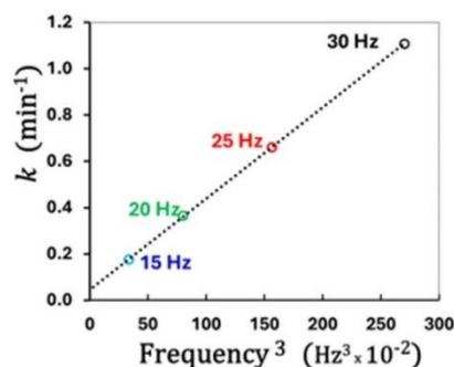
Figure 53 ) k , the volume fraction of powder effectively affected by CLCs (critical loading conditions) per unit time, as a function of the third power of the milling frequency, f^3 . Experiments milled under NG at 15 Hz, 20 Hz, 25 Hz and 30 Hz. Data has been taken from the kinetic studies summarised in Figure 52. 52, 73 Adapted from ref. 73 with permission from [RSC], copyright [2021] and figure drawn with original data supplied by Maria Carta.
