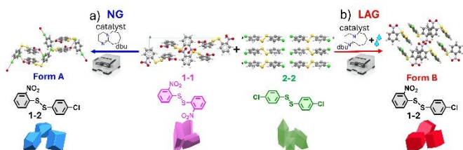
Figure 6 Model reaction used to probe ball milling trends. Base-catalysed (DBU) disulfide exchange between equimolar 1–1 and 2–2 yields the heterodimer 1–2. (a) Neat grinding (NG) produces polymorph Form A. (b) Liquid-assisted grinding (LAG) produces polymorph Form B. 41
