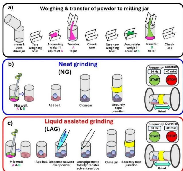
Figure 5: Protocol steps for the execution of ball mill reactions. a) Weighing and careful transfer of powder of the 2 starting materials (A and B) to the milling jar; b) and c)
