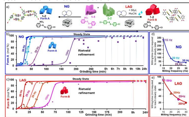
Figure 52 Effect of milling frequency on reaction kinetics of 1-1 + 2-2 with DBU forming 1-2. (a) Reaction scheme. (b) NG kinetics forming only Form A: 15 Hz grinding gives poor mixing and low reproducibility. (c) LAG kinetics (50 \mu\text{L} MeCN) forming only Form B. Each point represents an independent experiment. (d, e) Time to steady-state vs. frequency for NG (d) and LAG (e); lower frequencies require exponentially longer times. 52 Adapted from Ref. [52, DOI: 10.3762/bjoc.15.120], under the terms of the CC BY 4.0 license.
