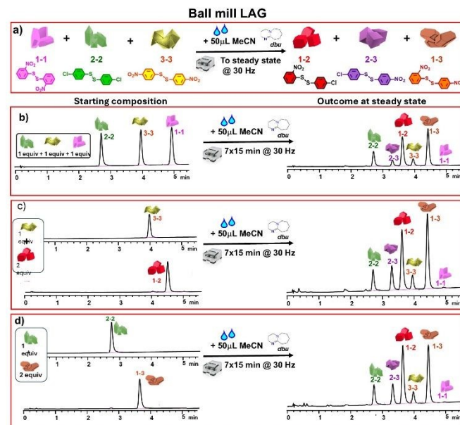
Figure 17 Steady-state composition under ball milling is independent of the starting point when overall stoichiometry is conserved. (a) Scheme of the equimolar LAG reaction of 1-1, 2-2, and 3-3 with DBU to steady-state, forming heterodimers 1-2, 1-3, and 2-3. (b-d) The same steady-state molecular distribution is reached whether starting from: (b) 1 equivalent each of 1-1, 2-2, and 3-3; (c) 2 equivalents of 1-2 plus 1 equivalent of 3-3; or (d) 2 equivalents of 1-3 plus 1 equivalent of 2-2. 41 Adapted from ref. 41 with permission from The Royal Society of Chemistry.
