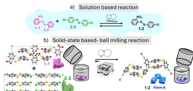
Figure 1 Visual conception of a disulfide exchange reaction scheme under a) solution-based conditions using molecular structures of the homodimers (1-1, 2-2) and the heterodimer (1-2) dissolved in a solvent (in light blue); b) under ball milling conditions depicting the crystal structures of the starting materials (1-1 and 2-2) and products involved (Form A polymorph of 1-2).
