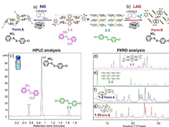
Figure 8 Synthetic scheme of ball mill disulfide exchange reaction under a) NG and b) LAG conditions. Analysis of the products. c) by HPLC analysis and d) to g) by PXRD analysis showing PXRD patterns corresponding to crystal structures of (d) 1–1, (e) 2–2, and the polymorphs of the heterodimer 1–2 as (f) Form A and (g) Form B. 41, 44
