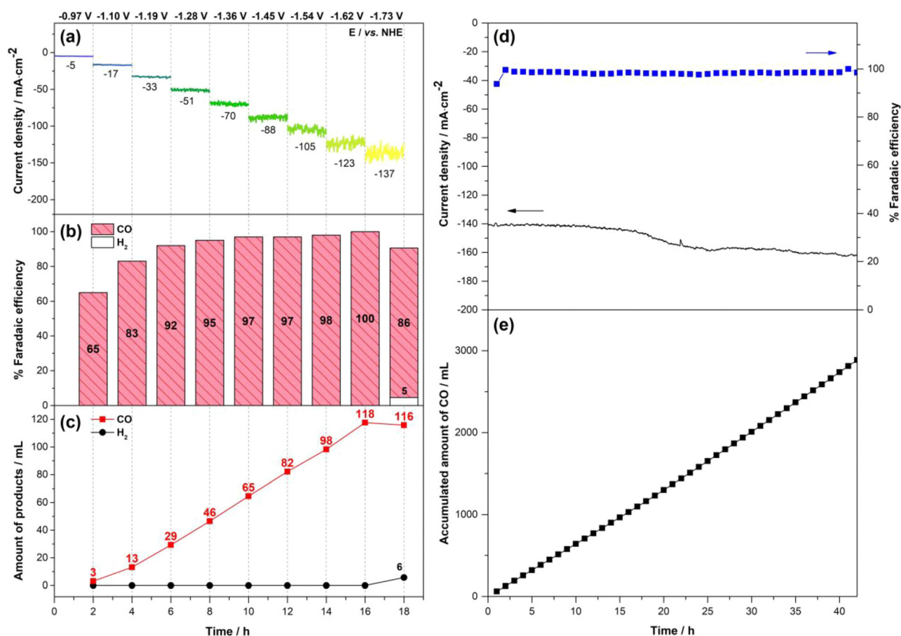
Fig. 7 (a) Chronoamperometric responses, (b) % FE of gas product formation and (c) accumulated amounts of CO (red line) and \text{H}_2 (black line) observed in each 2-h interval at various potentials; and (d) chronoamperometric responses with % FE CO and (e) accumulated amount of CO recorded at -1.54 \text{ V vs. NHE} over 42 h of the p(CoPc-1 \alpha )-catalyzed \text{ECO}_2\text{R} in the flow cell.
