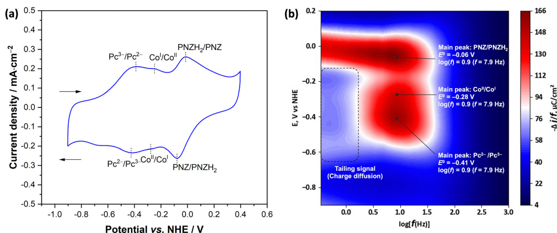
Fig. 4 (a) Cyclic voltammogram and (b) experimentally recorded VF-SWV colormaps of p(CoPc-1 \alpha )/CP , based on 76 square wave voltammograms collected with pulse times from 0.4 \mu s to 1.5 s, or the frequencies ( f ) from 1250 to 0.33 Hz in the region corresponding to Co II /Co I and Pc 2− /Pc 3− reduction processes.
