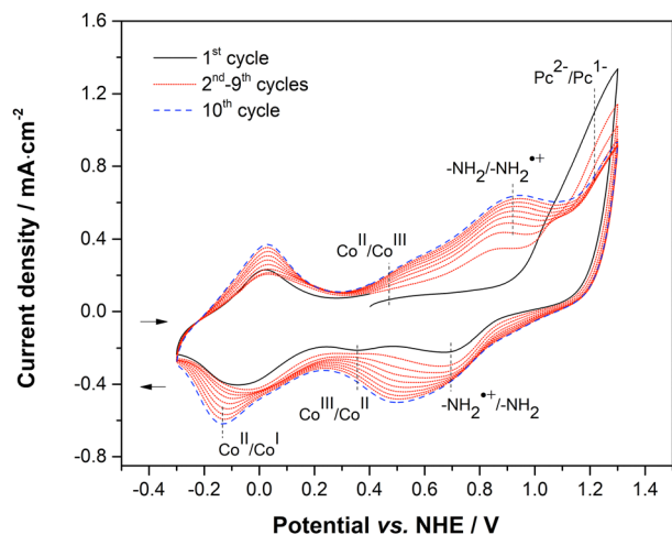
Fig. 2 The cyclic voltammograms of the electrochemical polymerization of CoPc-1α on the CP. Black solid, red dotted and blue dashed lines represent the first, the intermediate and the last scanning cycles, respectively.
