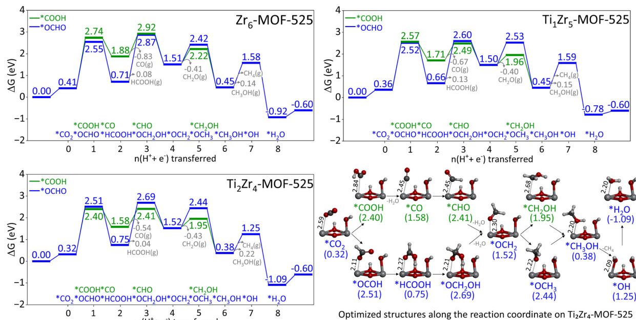
Fig. 2 Gibbs free-energy profiles ( \Delta G , eV) for the OH-passive pathway on Zr_6 -, Ti_1Zr_5 -, and Ti_2Zr_4 -MOF-525 clusters. The reactant state (MOF + CO_2 ) is used as the energy reference, and water desorption regenerates the active site. Optimized structures along the reaction coordinate are shown for the Ti_2Zr_4 -MOF-525, while those for Zr_6 - and Ti_1Zr_5 -MOF-525 are provided in the SI.
