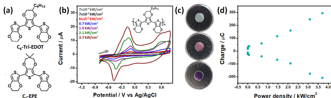
Fig. 2 (a) Chemical structures of C 6 -Tri-EDOT and C 2 -EPE. (b) Potentiodynamic characterization of poly-C 6 -Tri-EDOT films deposited on Pt electrodes as a function of P_{\text{hv}} (indicated in the figure) for a constant t_{\text{hv}} (10 min), obtained in a monomer-free 0.1 M TBAP/ACN solution, v = 50 mV s -1 . (c) Optical pictures of the electrode surface obtained before (top) and after electropolymerization of C 6 -Tri-EDOT (middle) and C 2 -EPE (bottom) at a constant P_{\text{hv}} and t_{\text{hv}} (2.1 kW cm -2 and 10 min, respectively). (d) Q_a and Q_c variation as a function of P_{\text{hv}} used for the light-driven electrocatalytic polymerization of C 6 -Tri-EDOT.
