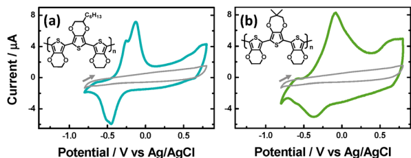
Fig. 3 Potentiodynamic characterization of (a) poly-C 6 -Tri-EDOT and (b) poly-C 2 -EPE films deposited on Pt electrodes with a constant P_{\text{hv}} ( 4.2 \times 10^{-3} \text{ kW cm}^{-2} ) and t_{\text{hv}} (30 min under mobile phone light), obtained in a monomer-free 0.1 M TBAP/ACN solution, v = 50 \text{ mV s}^{-1} .
