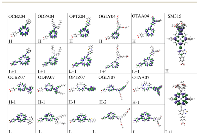
Fig. 5 Most contributing pairs of orbitals involved in the strongest one photon absorption peak in all the designed dyes, calculated at the TD-CAM-B3LYP/6-311+G(d,p)/C-PCM level of theory in acetonitrile solvent.
