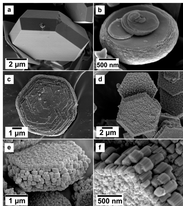
Fig. 15 SEM images illustrating the morphologies of (a) of La- and (b) Nd-fluorite crystals formed after fluorite ( \text{CaF}_2 ); (c and d) progressive replacement of the fluorite surfaces by REE-carbonates; (e and f) subsequent replacement of fluorite into Nd-bastnäsité at 200 °C forming pseudomorphic crystalline nanoaggregates.
