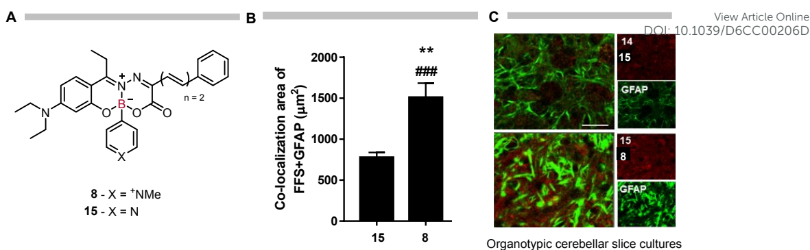
Figure 16. A) Structure of the BASHY dyes 8 (cationic) and 15 (neutral); B) Percentage of dye area that co-stains with GFAP; C) Representative images of slices stained with BASHY dyes 8 and 15 (red) and immunostained for GFAP (green). Adapted from ref. 63 with permission from John Wiley and Sons, Copyright 2020.
