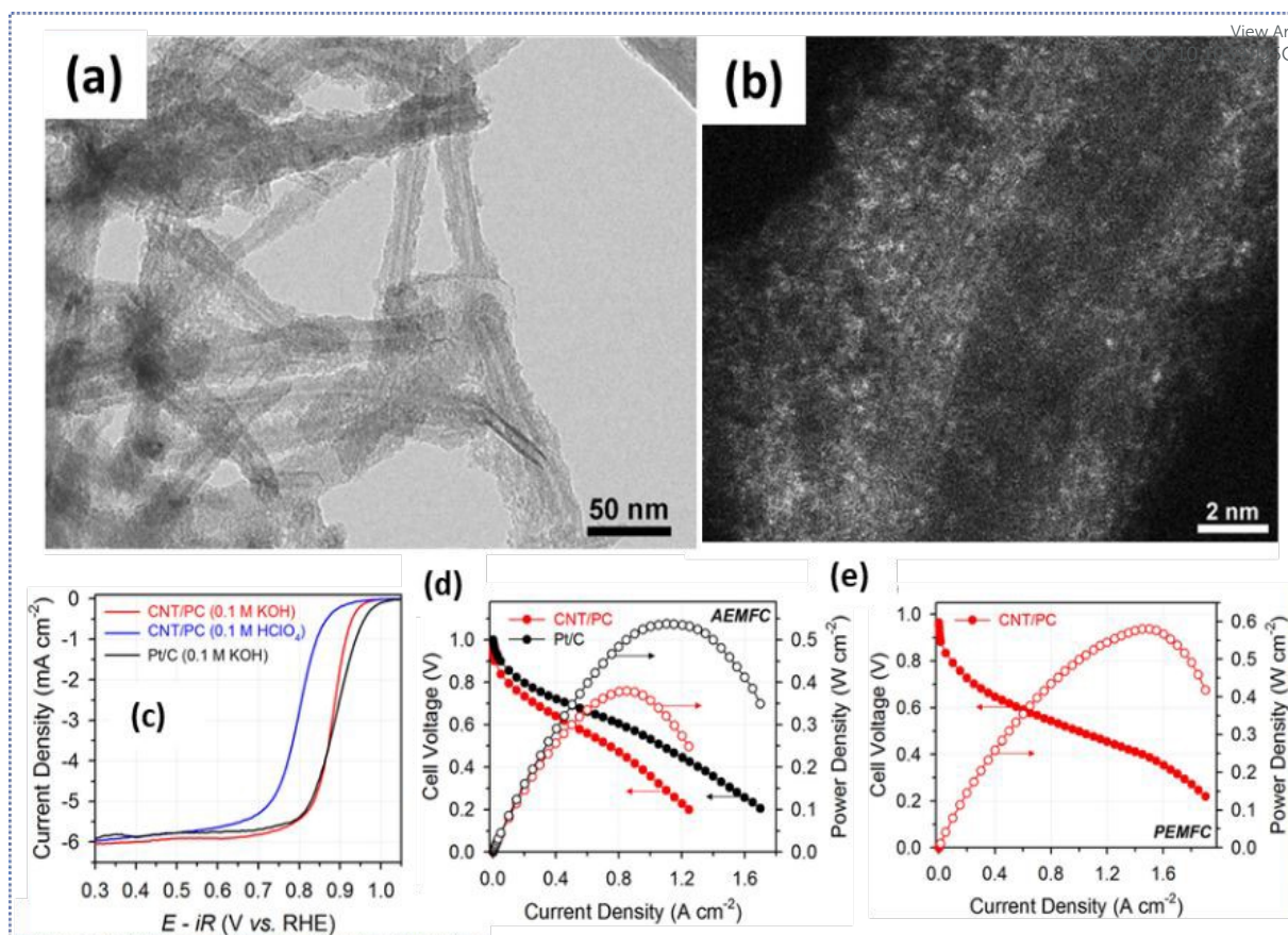
Fig. 6. (a) TEM and (b) HAADF-STEM image of CNT/PC. (c) ORR activity of CNT/PC. (d) AEMFC performances using CNT/PC and Pt/C catalysts, and (e) PEMFC performance with CNT/PC cathode catalyst. Reproduced from ref. 111 with the permission from the American Chemical Society, copyright 2016.
