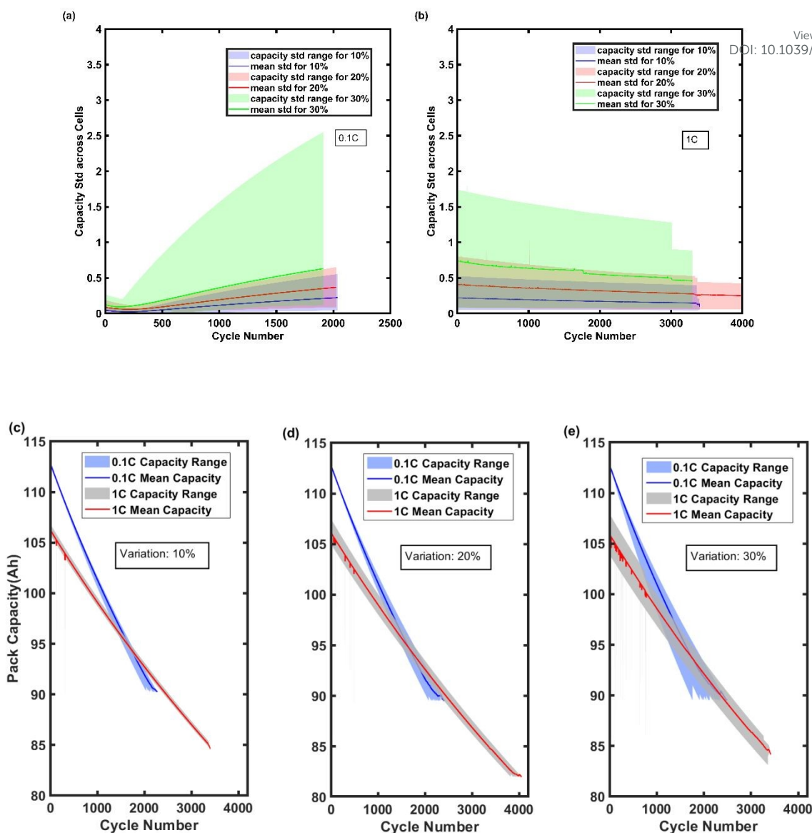
Fig. 4: Capacity analysis of 1S4P electrical configuration of battery pack. Panels (a, b): spread of capacity across cells at 0.1C and 1C, showing mean and standard deviation ranges for all three variation levels (i.e., 10%, 20%, 30%) over cycles. Panels (c-e): pack capacity degradation at 0.1C and 1C for 10%, 20%, and 30% capacity ranges over cycle life
