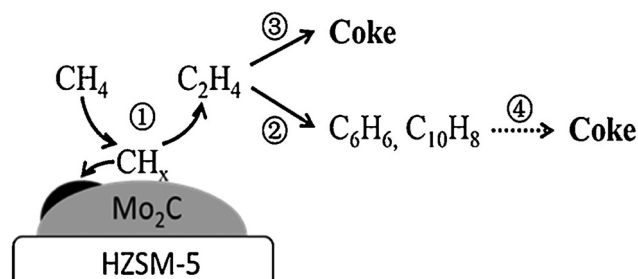
Fig. 12 Schematic diagram of coking pathways during \text{CH}_4 conversion over \text{Mo}_2\text{C}/\text{HZSM-5} catalyst. Reproduced from ref. 68 with permission from Elsevier, copyright 2014.
