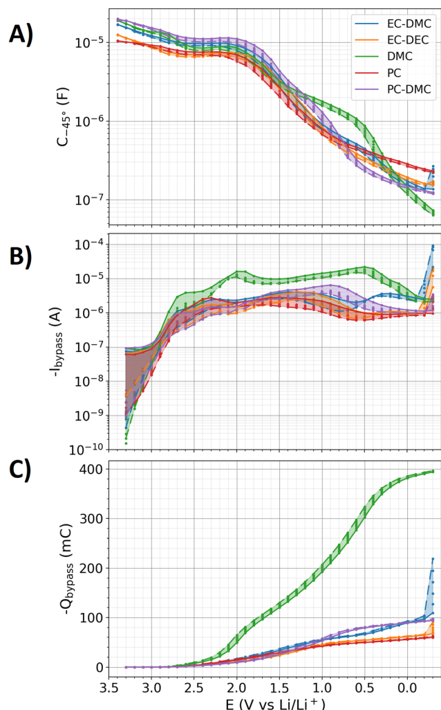
Fig. 4 Metrics derived from the impedance and amperometry measurements of the step protocol (see Fig. 1A), which show the potential and time-dynamics of the SEI formation. The total time for each measurement was approximately 16 hours. Colors: different electrolytes. Points: values extracted from 222 individual impedance spectra and amperometry measurements (37 different potential stages with each 6 iterations in time) for each electrolyte, respectively. Solid lines: values of the first iteration. Dashed lines: values of the sixth iteration. Shaded colored areas: data-span between the first and sixth iteration of the measurements. (A) Capacitances extracted from the impedance spectra. (B) Bypass currents extracted from the amperometry measurements. (C) Charges derived from integrated bypass currents.
