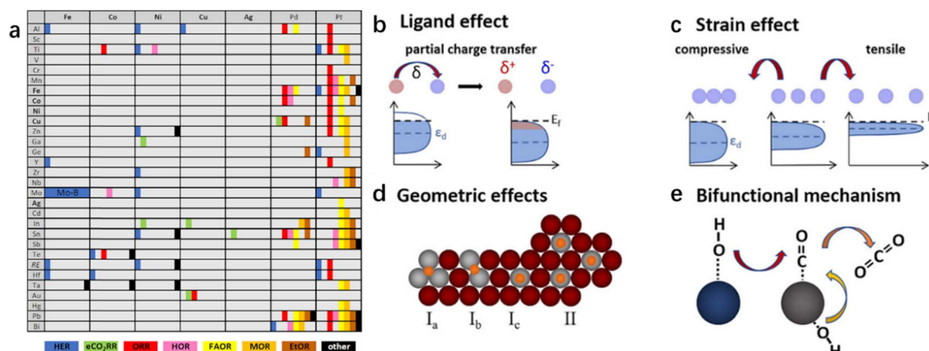
Fig. 2 (a) Overview of bimetallic systems and electrochemical reactions contained in this review. Bold elements appear in rows and columns to enable a concise scheme. RE stands for rare earth elements. "Other" reactions are electrochemical oxidation reactions of higher alcohols, \text{BH}_4^- , hydrazine, and methane and the oxygen evolution reaction (OER). Summarized optimization strategies: (b) ligand effects, (c) strain effects, (d) geometric effects, and (e) the bifunctional mechanism. (d) Geometric effects are divided into two parts. The first is the site isolation effect, accompanied by different adsorption possibilities of a molecule, that is, ( I_a ) in the hollow site, ( I_b ) on the bridge site or ( I_c ) on top of an atom. (II) The second is the equality of sites. 16 Reproduced with permission from ref. 16 Copyright 2019, ACS.
