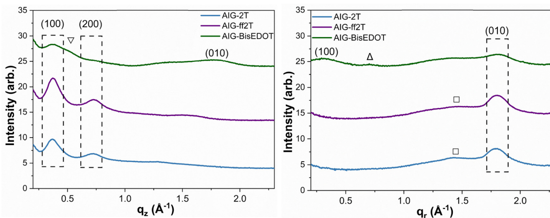
Fig. 6 GIWAXS out-of-plane ( q_z ) line cuts for AIG-2T , AIG-ff2T , and AIG-bisEDOT and in-plane ( q_r ) line cuts for AIG-2T , AIG-ff2T , and AIG-bisEDOT thin films; all films were annealed at 90 °C for 30 min.
