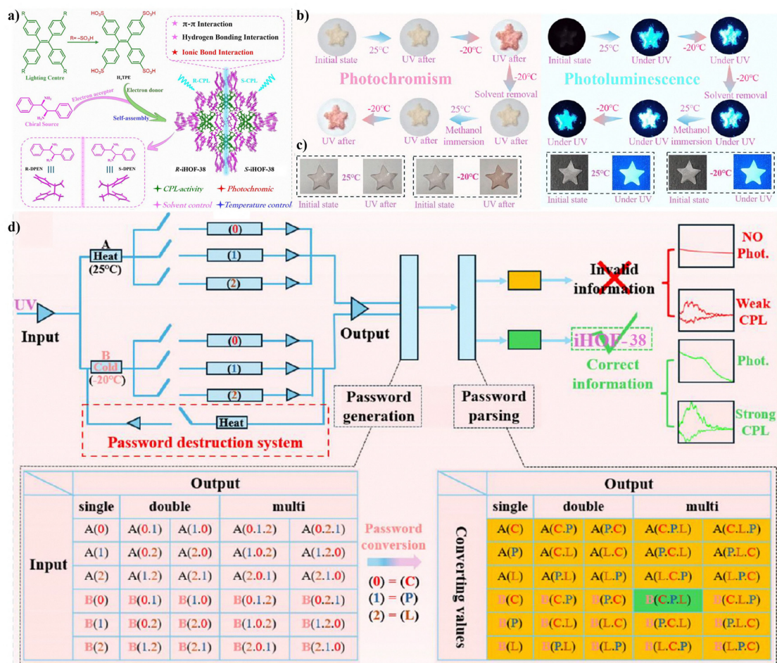
Fig. 24 (a) Chromophore tetrakis(4-sulfophenyl)ethylene (H4TPE), chiral source building blocks R / S -DPEN and R / S -iHOF-38 constructs and supra-molecular structures. (b) Photographs of the discoloration process under UV (365 nm), temperature-gated and solvent-controlled as well as fluorescence at different temperatures. (c) Photographs of discoloration and fluorescence of PVA composite films under UV (365 nm) conditions at different temperatures. (d) A multiple stimulus information encryption logic system was designed using UV = 365 nm as the stimulus source. Reproduced with permission from ref. 69. Copyright 2025, Wiley-VCH.
