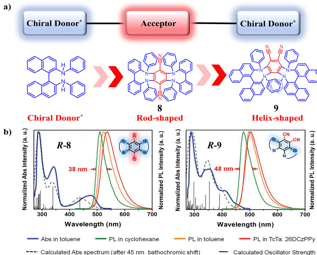
Fig. 5 (a) CP-TADF materials studied based on the D^*-A-D^* skeleton strategy. (b) The UV-vis absorption and PL spectra of R-8 and R-9 . Reproduced with permission from ref. 34. Copyright 2021, Wiley-VCH.
