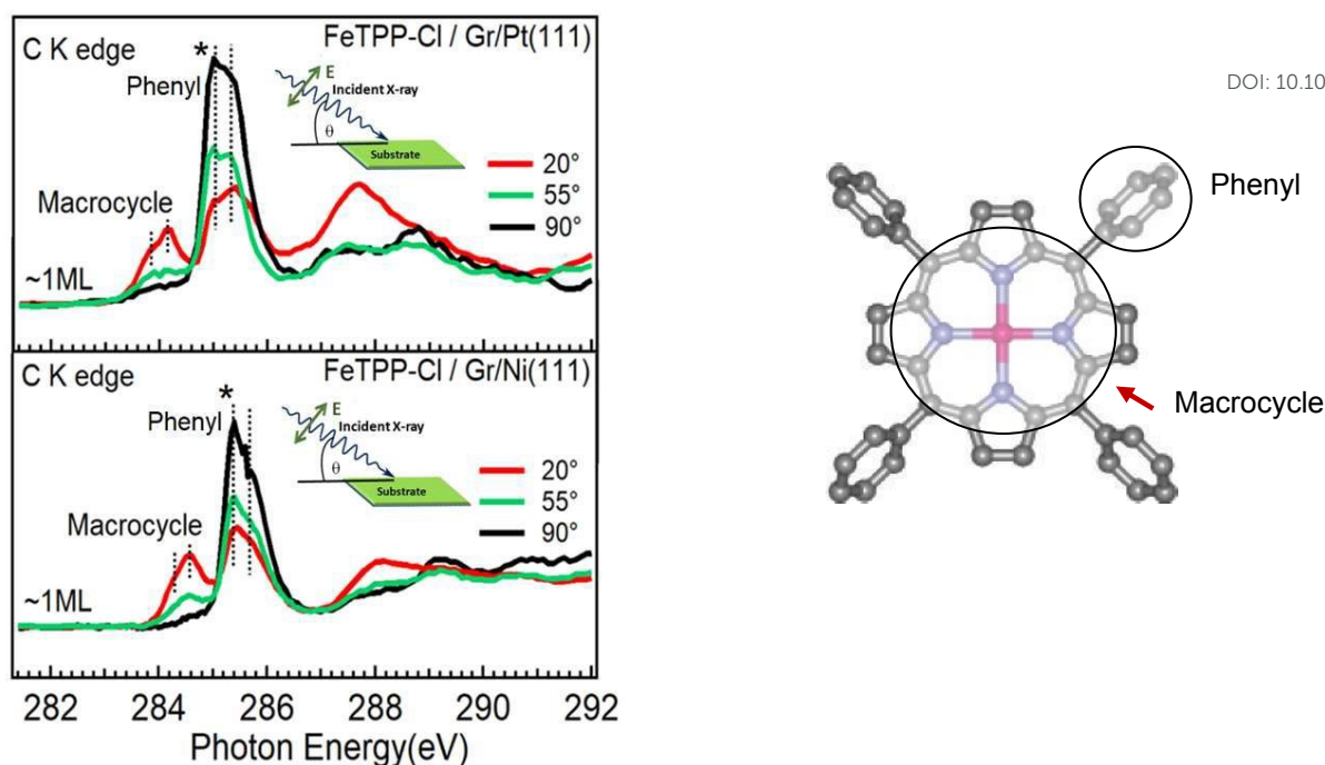
Figure 1 Left: C K-edge of 1 ML FeTPP-Cl/Gr/Pt(111), upper panel, and FeTPP-Cl/Gr/Ni(111), lower panel. The spectra have been obtained after subtraction of the bare graphene measurements. At normal incidence ( 90^\circ ), the data were acquired with the incoming photons perpendicular to the sample surface, resulting in the polarization vector lying parallel to the surface plane. At grazing incidence ( 20^\circ ), the photons arrive at the surface at a shallow angle, with the polarization vector oriented nearly perpendicular to the surface plane. Right: Structure of the tetraphenyl porphyrin, the circles indicate the central macrocycle and the external phenyl groups.
