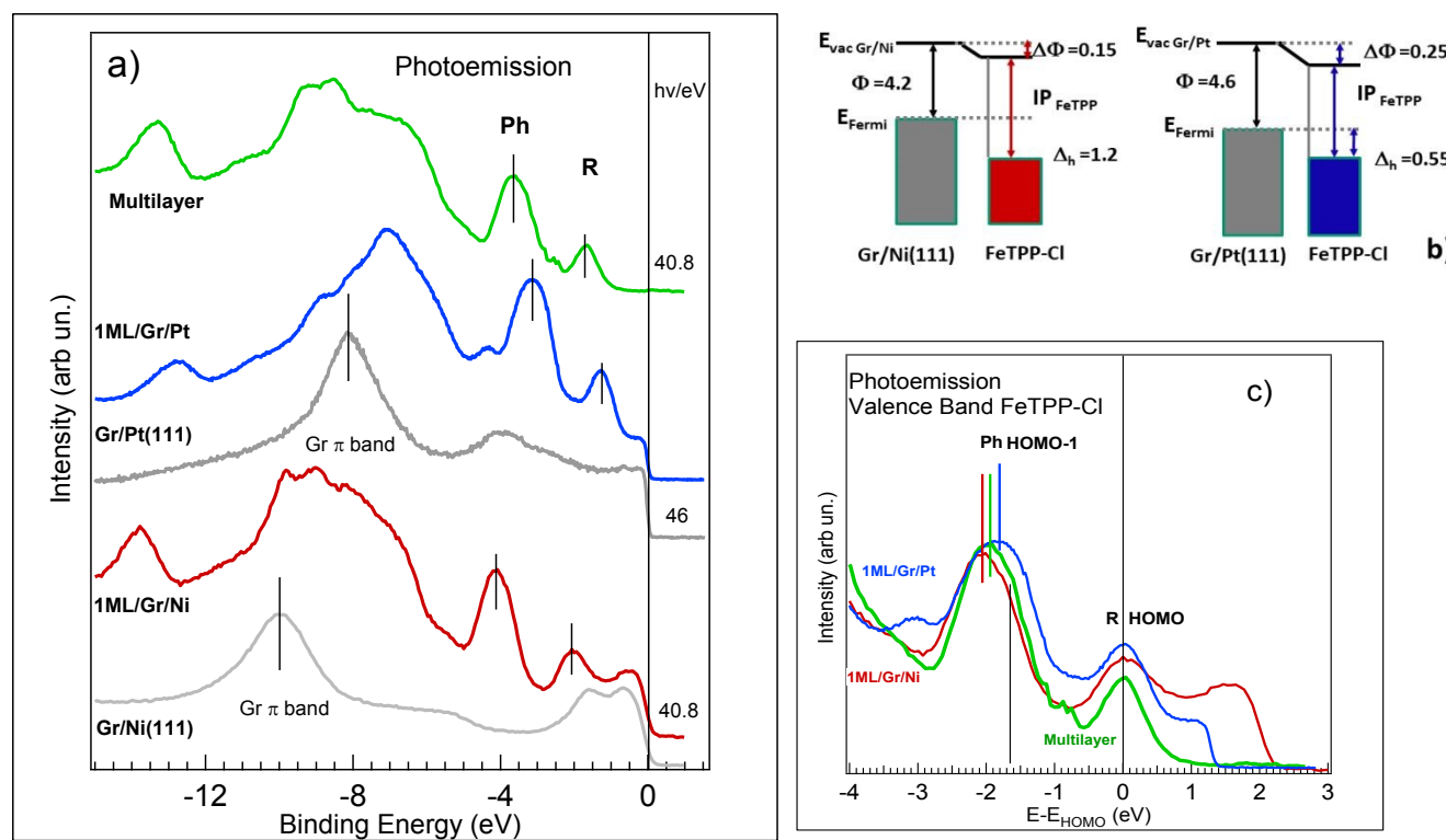
Figure 2. a) Valence band spectra of FeTPP-Cl multilayer (green), 1 ML FeTPP-Cl/Gr/Ni(111) (red), and FeTPP-Cl/Gr/Pt(111) (blue). Graphene spectra on Ni and Pt are shown in grey. \pi -band positions at 10.0 eV (Ni) and 8.1 eV (Pt) reflect doping differences. The photon energies used for the different spectra are indicated. b) Schematic representation of energy level alignment and hole injection barriers for the deposition of FeTPP-Cl on Gr/Ni(111), and Gr/Pt(111) in the monolayer regime. c) Zoom-in of HOMO-HOMO-1 region showing relative shifts and peak separations, FeTPP-Cl Multilayer (green curve), and 1 ML FeTPP-Cl (red and blue curves), energies are relative to the HOMO peak.
