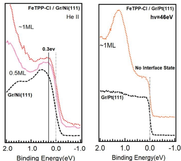
Figure 3. Valence band spectra close to the Fermi level for the 1 ML FeTPP-Cl on Gr/Ni(111) (Left) and Gr/Pt(111) (right). An interface state I_s is observed at 0.3 eV for FeTPP-Cl/Gr/Ni(111).
