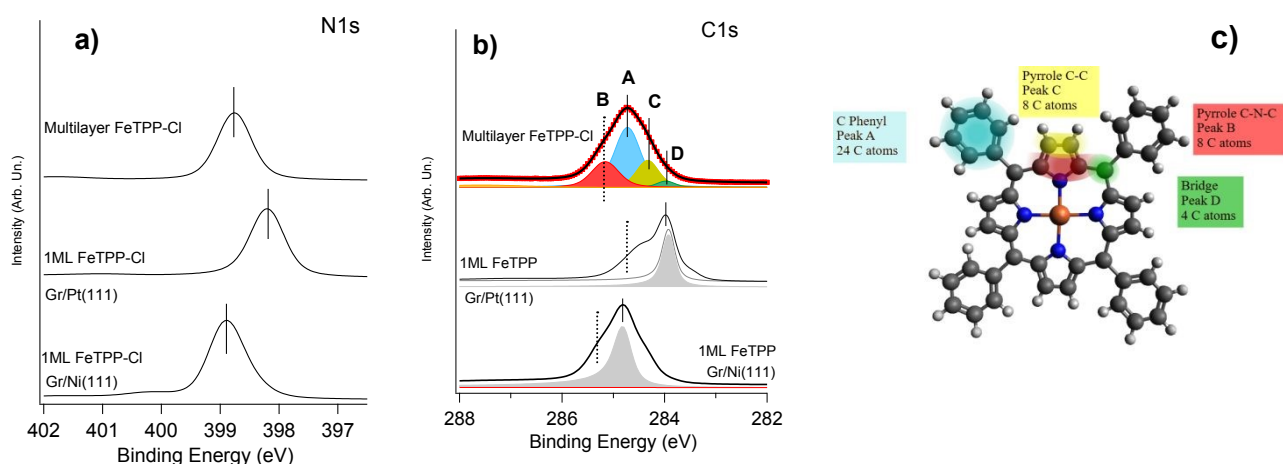
Figure 4. a) N 1s and b) C 1s photoemission spectra taken at h\nu=525 eV of multilayer and 1 ML FeTPP-Cl on Gr/Ni(111) and Gr/Pt(111). The feature labeled B in the b) panel indicates the B (pyrrole C-N-C) component obtained from fitting procedures. Tetraphenylporphyrins consist of four peripheral phenyl rings linked to the central tetrapyrrolic macrocycle. See text for details.
