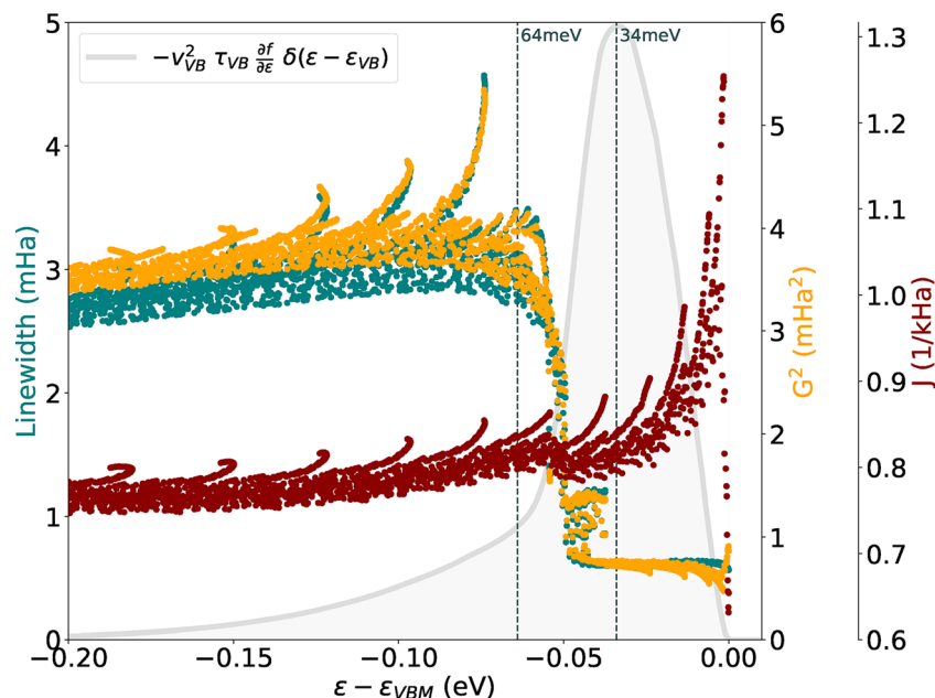
Fig. 4 Hole linewidths (in teal) near the VBM of SnO. The two parameters, G^2 and J , resulting from the decoupling of the scattering rates are also shown in orange and red, respectively ( \frac{1}{J} = G_{nk}^2 \times J_{nk} ). The grey area represents the function -v_{VB}^2 \tau_{VB} \frac{\partial f}{\partial \epsilon} \delta(\epsilon - \epsilon_{VB}) where v_{VB} and \tau_{VB} stand for the carrier velocity and lifetime in the VB, \frac{\partial f}{\partial \epsilon} is the derivative of the Fermi–Dirac distribution function with respect to the energy and \delta the Dirac delta function. By integrating this function, the relaxation time approximation (RTA) hole mobility is obtained. In other words, only the electronic states present under this curve participate in the hole transport of SnO.
