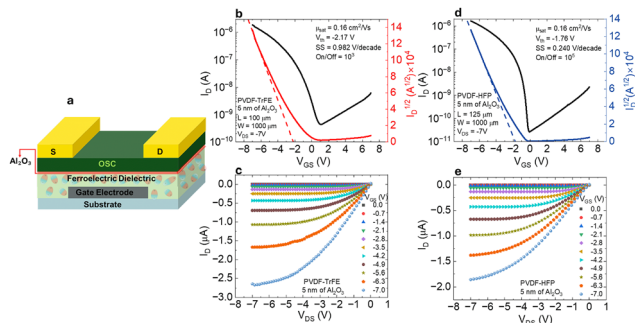
Fig. 4 FET characteristics with 5 nm \text{Al}_2\text{O}_3 . (a) Device geometry with the addition of \text{Al}_2\text{O}_3 layer. (b) and (c) Transfer and output characteristics of a DPP-DTT/PVDF-TrFE FET, respectively. (d) and (e) Transfer and output characteristics of a DPP-DTT/PVDF-HFP FET, respectively.
