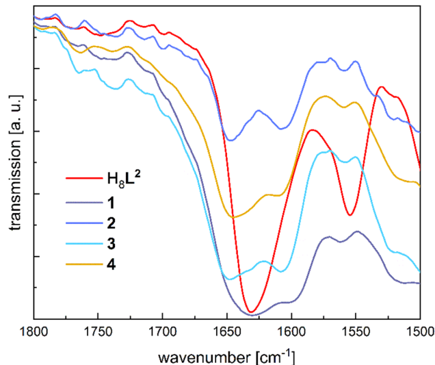
Fig. 2 Section of the ATR-FTIR Spectra of \text{H}_8\text{L}^2 and the complexes 1–4 in the 1800\text{--}1500\text{ cm}^{-1} region.
