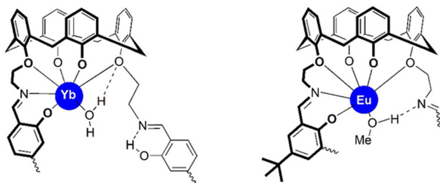
Fig. 8 Comparison of the immediate coordination environments in [\text{Yb}_2(\text{H}_2\text{L}^2)(\text{H}_2\text{O})_2] ( 4 ) (left) and in [\text{Eu}_2(\text{L}^1)(\text{MeOH})_2] (right). Parts of the structures were omitted for clarity.
