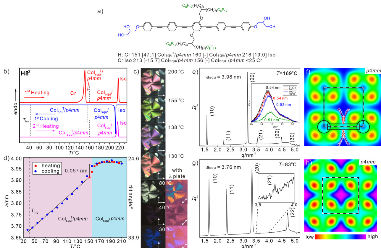
Fig. 2 (a) Formula of H8 2 with transition temperatures ( T/^\circ C ) and transition enthalpies ( \Delta H/kJ mol^{-1} ), (b) DSC traces, (c) textures as observed between crossed polarizers at the given temperatures, those at the very right are with additional \lambda -retarder plate, where blue fans in SW–NE direction indicate negative \Delta n and in NW–SE direction indicate positive \Delta n , for additional and enlarged textures, see Fig. S8 (ESI†); (d) a_{squ} = f(T) plot, the transition between tilted/non-tilted squares is indicated; (e) and (g) SAXS patterns at the given temperatures (for numerical data, see Tables S10 and S11, ESI†), inset in (e) shows the WAXS (for numerical data, see Table S2, ESI†) and (f), (h) ED maps reconstructed from these patterns (phase choices 000\pi for the first five peaks); lattice is shown by white dashed lines, tiles with molecules along edges are in black dashed lines and in (f) a molecular model is drawn according to the shape and size of H8 2 , black rectangle indicates the aromatic core and the black circles indicate the glycerol nodes.
