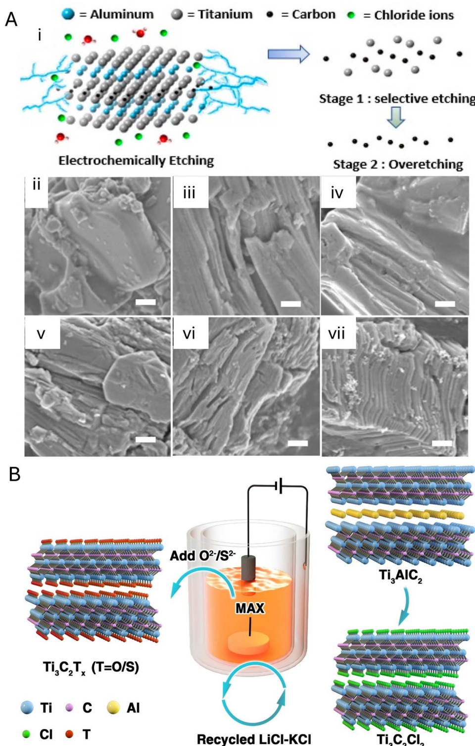
Fig. 8 (A) Electrochemical etching reaction mechanism and structural conclusions of the MXene \text{Ti}_2\text{CT}_x . (i) Anticipated electrochemical etching reaction mechanism route of the MAX phase \text{Ti}_2\text{AlC} in the HCl electrolyte solution. SEM micrographs of the MXene were obtained under varying HCl, temperature, time and voltage electrochemical etching conditions. (ii) MAX \text{Ti}_2\text{AlC} , (iii) 1 M/25 °C/9 h/0.3 V, (iv) 1 M/50 °C/3 h/0.3 V without CB, (v) 1 M/50 °C/3 h/0.3 V, (vi) 1 M/50 °C/6 h/0.3 V, and (vii) 1 M/50 °C/9 h/0.3 V. Scale bars: 1 \mu\text{m} . Reproduced with permission. 200 Copyright 2019, American Chemical Society. (B) Illustration of the fabrication process of MXene from the corresponding MAX phase through MS-electrochemical etching, followed by the in situ modification of surface terminations. Reproduced with permission. 172 Copyright 2021, Wiley-VCH.
