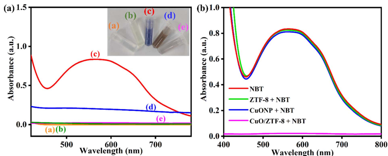
Fig. 3 Absorbance spectra of (a) \text{O}_2^{\bullet-} in DMSO (orange), (b) 1 \text{ mg mL}^{-1} of NBT in 0.1 \text{ M PBS (pH 7)} (green), (c) \text{O}_2^{\bullet-} –NBT system (red), (d) 0.5 \text{ mg mL}^{-1} of CuO/ZTF-8 in 0.1 \text{ M PBS (pH 7)} (blue), and (e) \text{O}_2^{\bullet-} –NBT system in the presence of CuO/ZTF-8 (pink). (Inset) Visual representation of the colour changes observed (b) \text{O}_2^{\bullet-} –NBT system in the absence (red) and presence of ZTF-8 (green), CuONP (blue), and CuO/ZTF-8 (pink) in 0.1 \text{ M PBS (pH 7)} .
