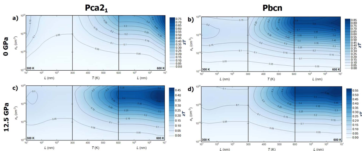
Fig. 7 Thermoelectric figure of merit ( zT ) for n-type BiN as function of temperature ( T ), carrier concentration ( n ) and averaged grain size ( L ). (a and b) zT for Pca2_1 and Pbcn polymorph at 0 GPa, respectively. (c and d) zT for Pca2_1 and Pbcn polymorph at 12.5 GPa, respectively.
