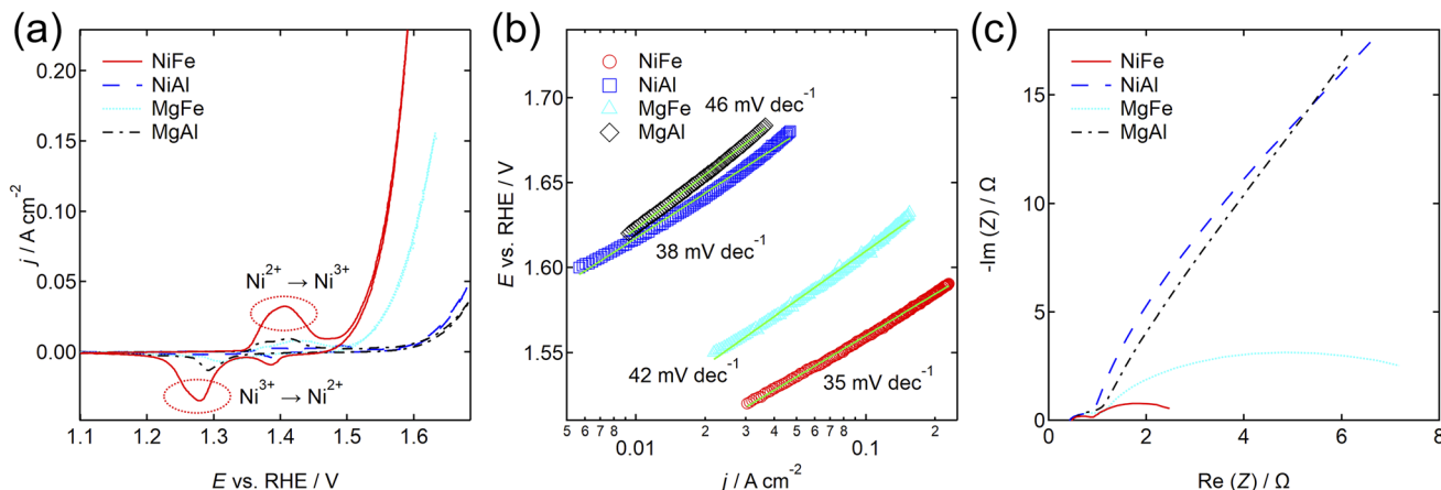
Fig. 2 (a) Cyclic voltammograms (CVs), (b) Tafel plots, and (c) Nyquist plots of NiFe-LDH/NF, NiAl-LDH/NF, MgFe-LDH/NF, and MgAl-LDH/NF in O_2 -saturated 1\text{ mol dm}^{-3} KOH. The scans were performed at a scan rate of 5\text{ mV}^{-1} in (a) and (b).
