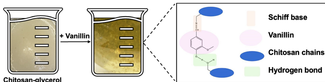
Fig. 1 Schematic of the synthesis of CVG cross linked films and the cross-linking mechanism.
