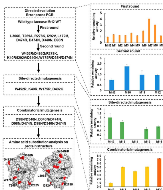
Fig. 23 Schematic diagram of laccase engineering through FACS-facilitated directed evolution. 154 Amino acid substitutions are shown in red colour. Copyright ACS, 2025.
