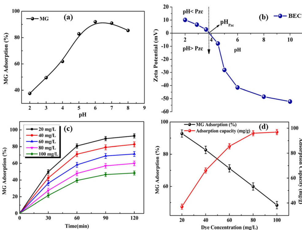
Fig. 7 (a) Effect of pH (adsorbent amount = 0.5 \text{ g L}^{-1} ; MG dye conc. = 20 \text{ mg L}^{-1} ; temperature = 25^\circ \text{C} ), (b) \text{pH}_{\text{PZC}} of the BEC adsorbent, (c) effect of adsorption time, and (d) effect of dye concentration on MG dye removal by the BEC adsorbent ( \text{pH} = 6 ; adsorbent amount = 0.5 \text{ g L}^{-1} ; contact time = 120 min; temp. = 25^\circ \text{C} ).
