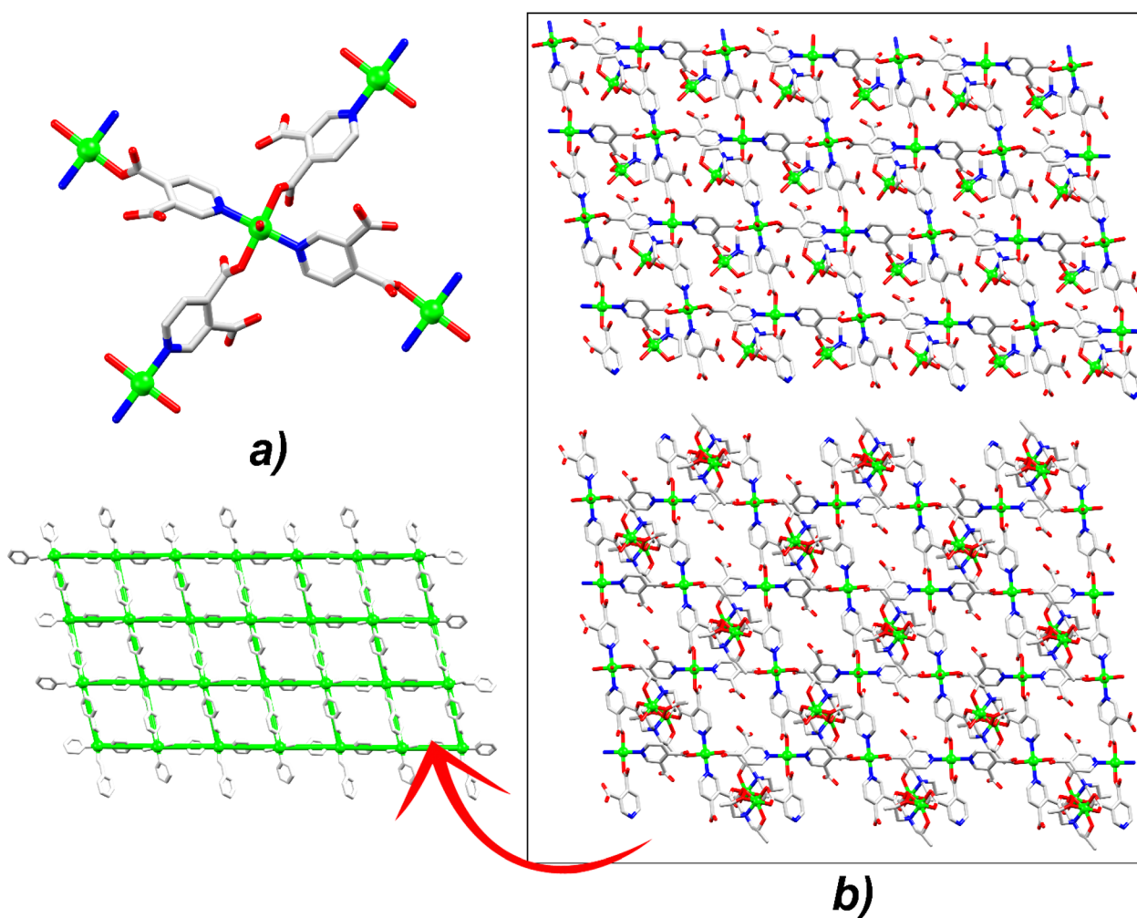
Fig. 3 (a) Illustration of 'central' \{\text{CuO}_3\text{N}_2\} blocks interconnected by four adjacent square pyramidal units through \text{pd}c^{2-} linkers in Cu-tipa (similar interconnections are seen in Cu-mdea , top). Color codes: Cu green balls, O red, N blue, C gray. (b) 2D metal-organic layers formed in Cu-mdea (top) and Cu-tipa (bottom) directed by the \{\text{CuO}_3\text{N}_2\} units. Topological representation of the simplified uninodal 4-connected underlying net with the \text{sql} topology; green balls are the centroids of the \{\text{CuO}_3\text{N}_2\} units.
