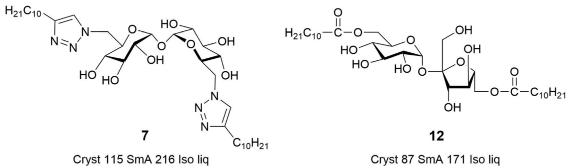
Fig. 18 Comparison between the temperatures ( ^{\circ}\text{C} ) of the phase transitions of compound 7 and 6,6'-di-O-undecanoylsucrose 12 .
