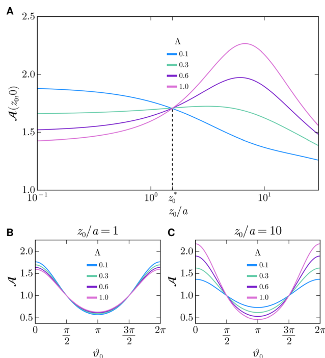
Fig. 5 (A) Anisotropy \mathcal{A}(z_0, 0) as a function of the initial position z_0/a for different resetting rates \Lambda . (B) and (C) Anisotropy as a function of the initial angle \vartheta_0 for different \Lambda and z_0/a . The Péclet number is Pe = 0.4 .
