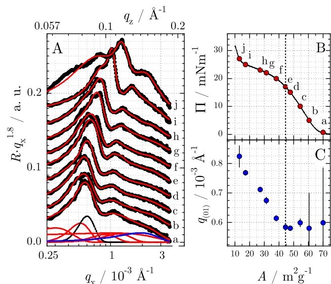
Fig. 4 A: q_x^{1.8} weighted in situ off-specular X-ray scattering of MG particles at the air-water interfaces at the pressures highlighted on the isotherm in panel B, starting from the bottom with the lowest lateral pressure. Black symbols are the measured values, and red solid lines are optimised models as described in the text. For improved visibility, the curves are shifted by 0.05 against each other. B: \Pi - A isotherm of the PNIPAM MG particles at the air/water interface (black solid line). Red symbols indicate the pressures at which the OSR were recorded. C: Centre positions of the fitted Gaussian representing the (01) peak.
