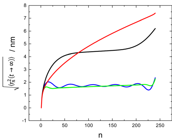
Fig. 7 Limiting square root segmental MSD ( \sqrt{\langle r_n^2(t \rightarrow \infty) \rangle} ) for heterogeneously relaxing chain ensembles as a function of monomer number along the chain; green and black lines: components from the site dependent friction approach; blue and red lines: topological constraints only. The grafting point is situated at n = 1 .
