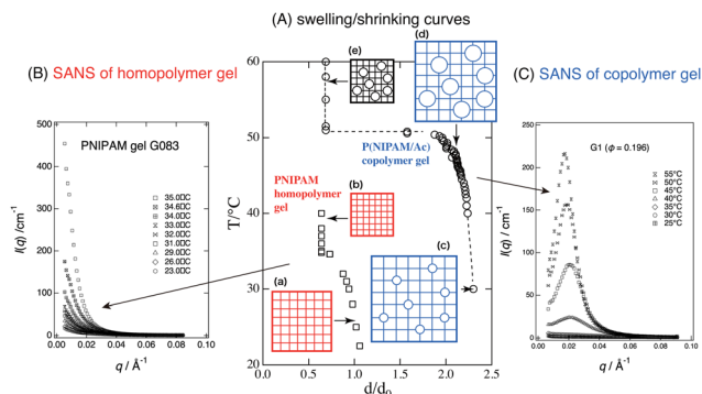
Fig. 7 Swelling/shrinking curves ( T vs. d/d_0 ) (A), and SANS profiles for PNIPAM (homopolymer) gel (B) and P(NIPAM/Ac) (copolymer) gel (C). Homopolymer gels undergo a continuous VPT, while copolymer gels undergo a discrete VPT. SANS of the former shows critical divergence at T_{\text{PNIPAM}} \approx 32 °C, while the latter shows a marked peak at T > T_{\text{PNIPAM}} . The cartoons of square grids and circles show PNIPAM networks and ionized chain regions associated with AAC comonomers, respectively. The cartoons indicate that the size of the gel (grids) becomes smaller via hydrophobic contraction and the circles become larger via electrostatic repulsion, with changing T . (Modified from parts of Fig. 2 in ref. 49.)
