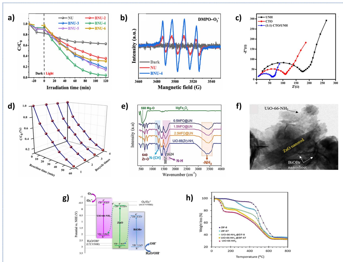
Fig. 12 (a) Photocatalytic degradation of TC by NU and BNU composites under vis-light irradiation, (b) ESR spectra of DMPO-·O 2 - for NU and BNU-4, reproduced with permission from Elsevier. Copyright © 2024. 117 (c) EIS analysis of UNH, CTO, and CTO@UNH (1:1), reproduced with permission from Elsevier. Copyright © 2020. 74 (d) Reusability test results of CTO@UNH (1:1), reproduced with permission from The Korean Institute of Chemical Engineers. Copyright © 2022. 118 (e) FTIR spectra of the samples, reproduced with permission from Elsevier. Copyright © 2023. 119 (f) TEM images of the ZBU heterojunction, reproduced with permission from Elsevier. Copyright © 2024. 121 (g) Z-scheme mechanism of ZnO/BiOBr/Uio-66-NH 2 charge transfer on TC degradation, reproduced with permission from Elsevier. Copyright © 2023. 119 (h) TGA curves of pristine Uio-66-NH 2 , ZIF-67, ZIF-8, and their composites, reproduced with permission from Wiley. Copyright © 2024. 121
