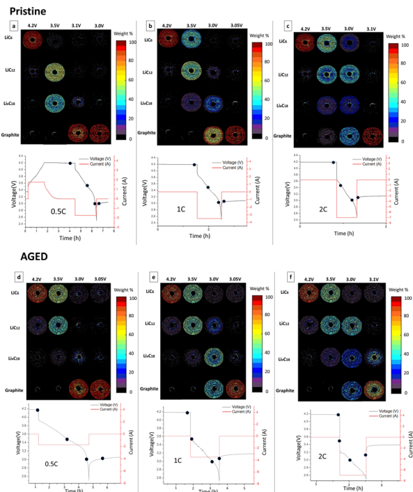
Fig. 6 Weight% distribution of different graphite phases during discharge at increasing C rates inside the pristine cell. Pristine cell is shown in (a)–(c), starting from a C rate of 0.5 to 2C. Aged cell is shown in (d)–(f), starting from a C rate of 0.5 to 2C.
