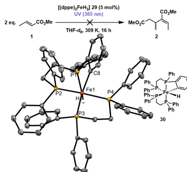
Scheme 3 Using [(dppe)_2FeH_2] 29 as catalyst for methyl crotonate 1 dimerisation under UV (365 nm) irradiation for 16 hours yielded no ( E ),( Z )-2-ethylidene-3-methylpentanedioate 2 . Crystals suitable for X-ray crystallography were grown from the reaction mixture at -35^\circ C and identified as [(dppe)FeH(Ph_2PCH_2CH_2PPh(C_6H_4))]_2 30 . Iron, carbon and phosphorus atoms on the molecular structures are coloured orange, grey and yellow respectively. Hydrogens have been omitted for clarity and thermal ellipsoids have been set at 50% probability.
