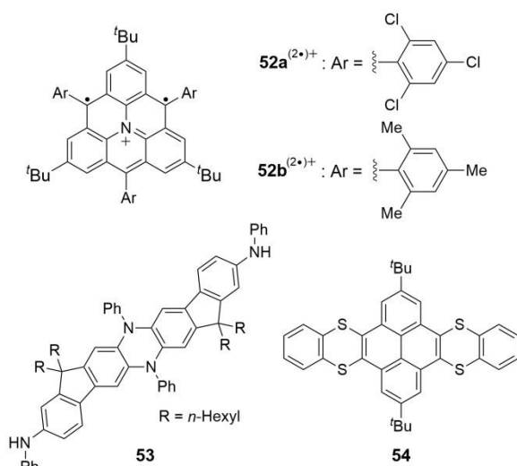
Fig. 17 Structures of cation 52a/b^{2(+)} and compounds 53 and 54 .
