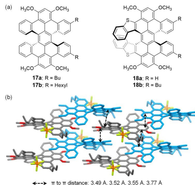
Fig. 6 (a) Double helixenes 17a/b and 18a/b ; (b) \pi - \pi stacking in the crystal of 17a •+ PF 6 − , where the ( M , M ) enantiomer is shown in blue, and the ( P , P ) enantiomer is colored according to the elements. Reproduced with permission from ref. 40. Copyright 2022 American Chemical Society.
