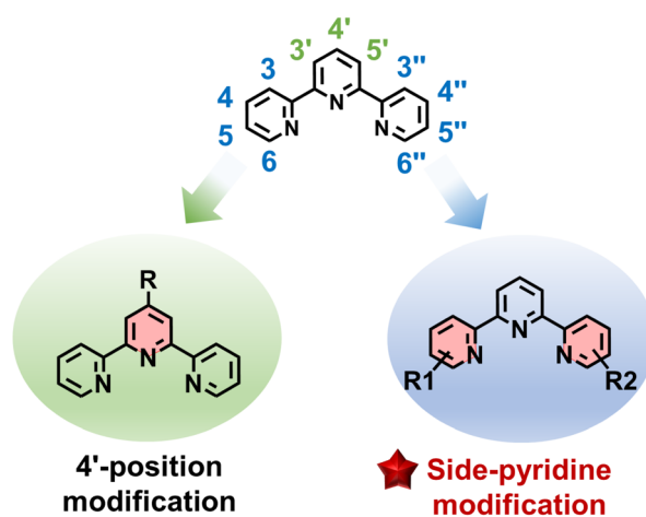
Fig. 1 The illustration of 4'-position and side-pyridine modifications of tpy.
