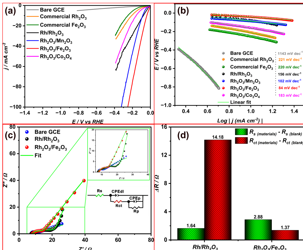
Fig. 5 (a) LSV curves recorded at a scan rate of 100 \text{mV s}^{-1} for commercial \text{Rh}_2\text{O}_3 , commercial \alpha\text{-Fe}_2\text{O}_3 , and synthesized Rh/Rh _2\text{O}_3 , Rh _2\text{O}_3/\text{Mn}_2\text{O}_3 , Rh _2\text{O}_3/\text{Fe}_2\text{O}_3 , and Rh _2\text{O}_3/\text{Co}_3\text{O}_4 in 0.5 M \text{H}_2\text{SO}_4 (without iR compensation); (b) corresponding Tafel plots derived from the LSV data; (c) Nyquist plots for Rh/Rh _2\text{O}_3 , Rh _2\text{O}_3/\text{Fe}_2\text{O}_3 , and bare GCE, with insets showing magnified semicircle regions and the equivalent circuit used for fitting; (d) comparative plot of charge transfer resistance ( \Delta R_{\text{ct}} ) values extracted from EIS data for Rh/Rh _2\text{O}_3 and Rh _2\text{O}_3/\text{Fe}_2\text{O}_3 relative to bare GCE.
