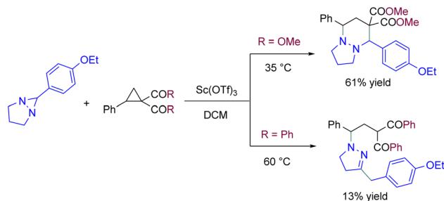
Scheme 1 Enantioselective reactions of diaziridines and representative pyrazoline-incorporating derivatives.
