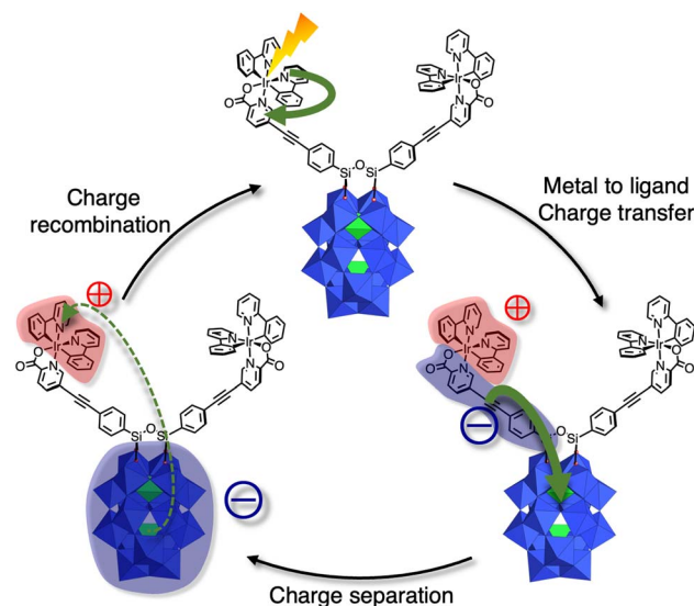
Fig. 5 Directionality in the photoinduced electron transfers of the POM-Ir(III) assembly [P_2W_{17}O_{61}\{O(SiC_{36}H_{23}O_2N_3Ir_2)\}]^{6-} , conferred by the heteroleptic character of the Ir(III) complex. The red and blue cloud respectively represent the localization of the positive and negative charges in the different excited states. 51
