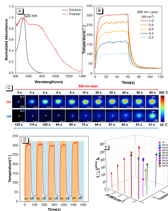
Fig. 4 (A) UV-vis-NIR spectra of PI in \text{DMSO} solution ( 10 \mu\text{M} ) and in the powder state. (B) Heating and cooling characteristics of PI powder under 808 nm laser irradiation at various power densities (0.2, 0.4, 0.6, 0.8, and 1.0 \text{ W cm}^{-2} ). (C) Thermal IR images of PI powder (15 mg) under 808 nm laser irradiation at 1.0 \text{ W cm}^{-2} , followed by turning off the laser. (D) Reversibility of PI powder (15 mg) under 808 nm laser irradiation at 1.0 \text{ W cm}^{-2} . (E) The highest temperature and corresponding time of the reported polymer organic photothermal materials under 808 nm laser irradiation.
