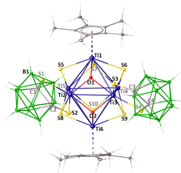
Fig. 1 Molecular structure and labelling diagram of 1. Cp* ligands attached to Ti4 and Ti5 atoms are omitted for clarity. Selected bond lengths (Å) and bond angles (°): Ti...Ti 3.130–3.598, Ti1–S5 2.4274(12), Ti1–O1 1.919(2), Ti2–S5 2.4835(12), Ti2–S1 1.3963(13), C1–S1 1.785(4), B1–C1 1.703(7), Ti3–Ti2–Ti5 93.913, Ti1–S5–Ti2 82.52(4).
