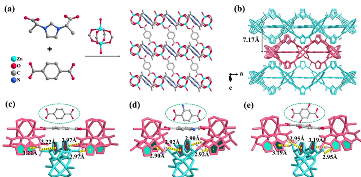
Fig. 1 (a) Diagrams illustrating the secondary building units and layer structures of L-1. (b) 3D stacking diagrams along the b -axis of L-1. (c)–(e) The C–H–π interaction between adjacent layers of L-1, L-2, and L-3.
