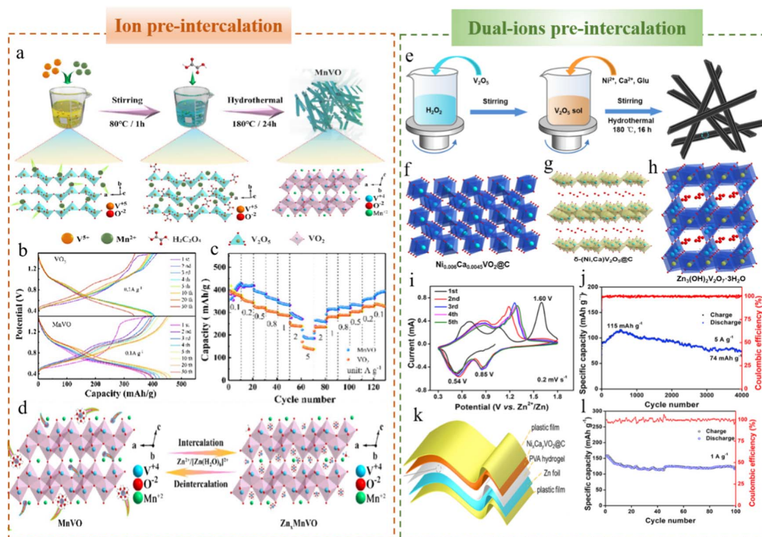
Fig. 11 (a) Schematic diagram of the synthesis of MnVO. (b) Charge–discharge curves and (c) rate performance curves of MnVO and \text{VO}_2 . (d) Schematic diagram of \text{Zn}^{2+} insertion/extraction of MnVO. 79 Copyright 2023, American Chemical Society. (e) Schematic diagram of the synthesis of \text{Ni}_{0.006}\text{Ca}_{0.0045}\text{VO}_2@\text{C} . Structures of (f) \text{Ni}_{0.006}\text{Ca}_{0.0045}\text{VO}_2@\text{C} , (g) \delta\text{-(Ni,Ca)V}_2\text{O}_5@\text{C} , and (h) \text{Zn}_3(\text{OH})_2\text{V}_2\text{O}_7 \cdot 3\text{H}_2\text{O} . (i) CV curve of \text{Ni}_{0.006}\text{Ca}_{0.0045}\text{VO}_2@\text{C} , (j) cycle diagram of \text{Ni}_{0.006}\text{Ca}_{0.0045}\text{VO}_2@\text{C} , (k) schematic diagram of the structure of a flexible quasi-solid-state battery, and (l) cycle performance diagram of the solid-state battery. 82 Copyright 2022, Elsevier.
