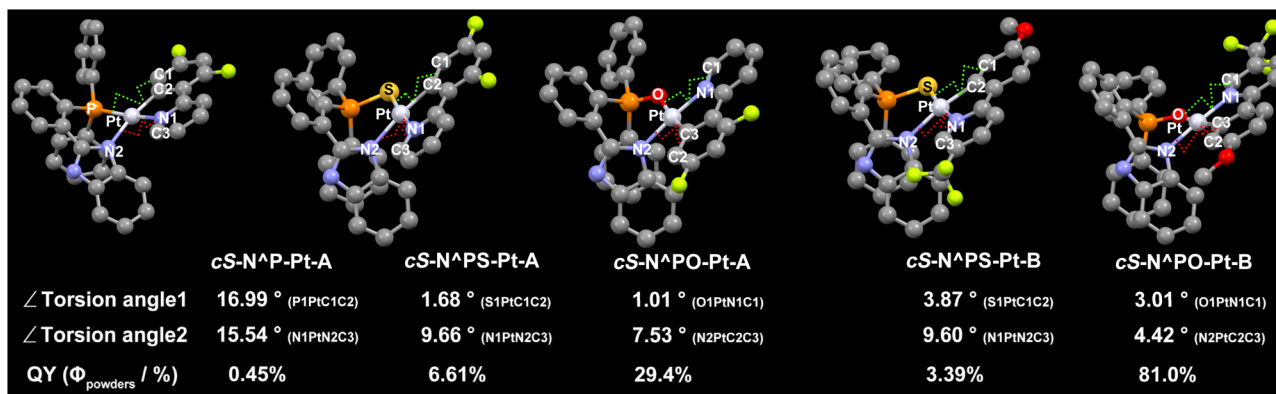
Fig. 7 The relationship between emission quantum yields and torsion angles of coordinated atoms among the representative products: cS-N P -Pt-A, cS-N PS -Pt-A, cS-N PO -Pt-A, cS-N PS -Pt-B, and cS-N PO -Pt-B.
