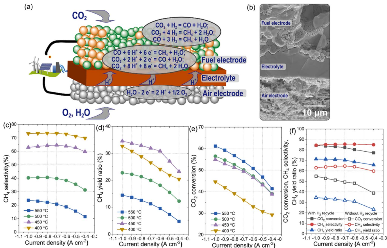
Fig. 19 (a) Schematic illustration of the possible electrochemical and chemical reactions during electrolysis and upgrading CO 2 –H 2 O into CH 4 in the PEEC (b), (c–e) one pass CO 2 conversion, CH 4 selectivity, and CH 4 yields at 400–550 °C, and (f) with H 2 recycling at 450 °C. 117 Reproduced with permission.
