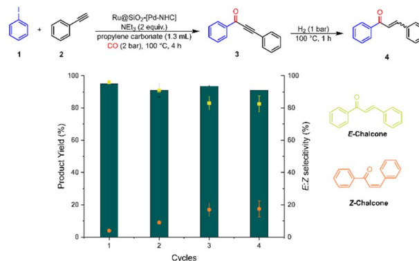
Fig. 7 Recycling experiments for the one-pot synthesis of chalcones 4 using Ru@SiO 2 -[Pd-NHC].
