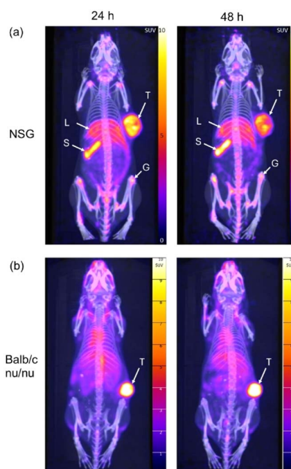
Fig. 3 Representative maximum intensity projection PET/CT images of SKOV-3 xenograft tumour-bearing (a) NSG and (b) Balb/c nu/nu mice, 24 and 48 h following administration with [ ^{64}\text{Cu} ]CuSar-trastuzumab. Tumour (T), liver (L), spleen (S) and growth plates (G) are indicated.
